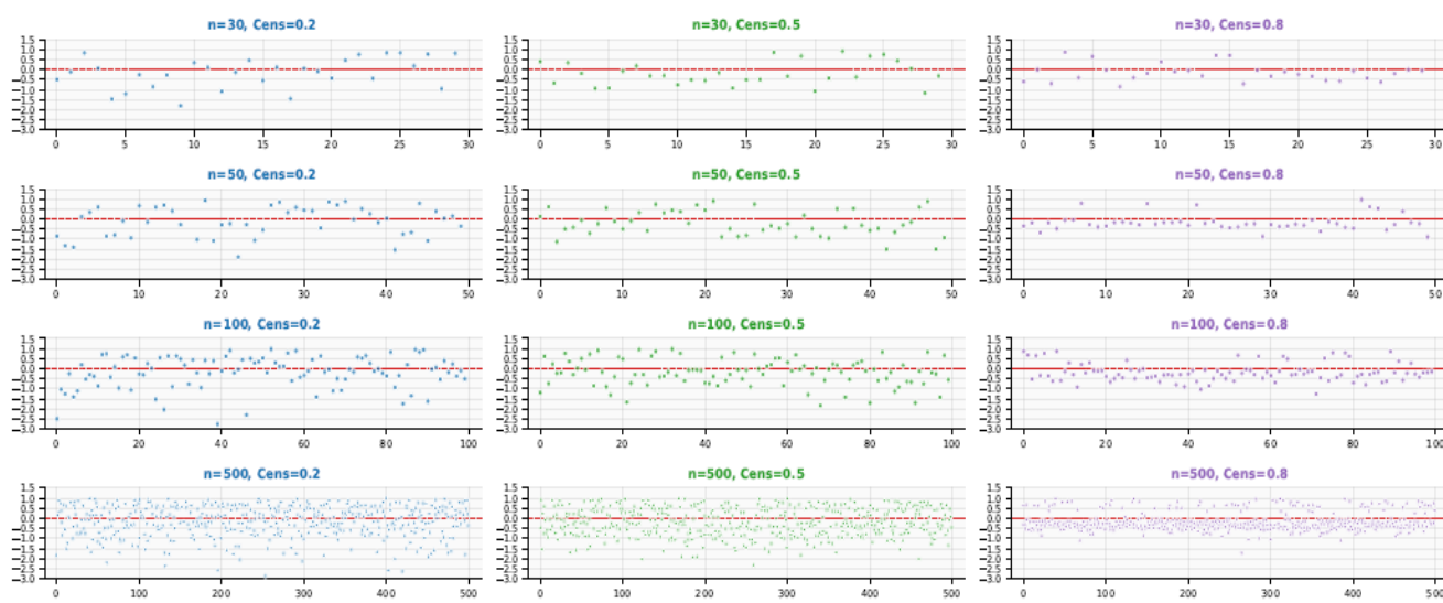
Figure 14. Martingale residuals grid (Case 3) for different sample sizes and censoring levels.
