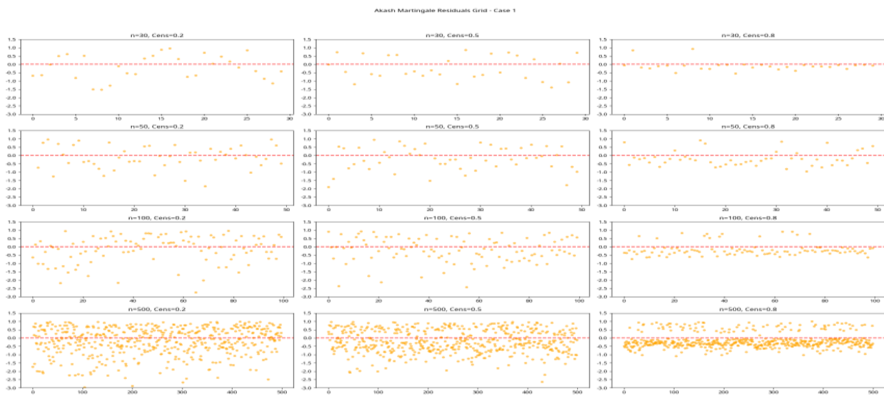
Figure 6. The Martingale residuals for the MG Akash Regression Model (Case 1) across different sample sizes and censoring levels.
