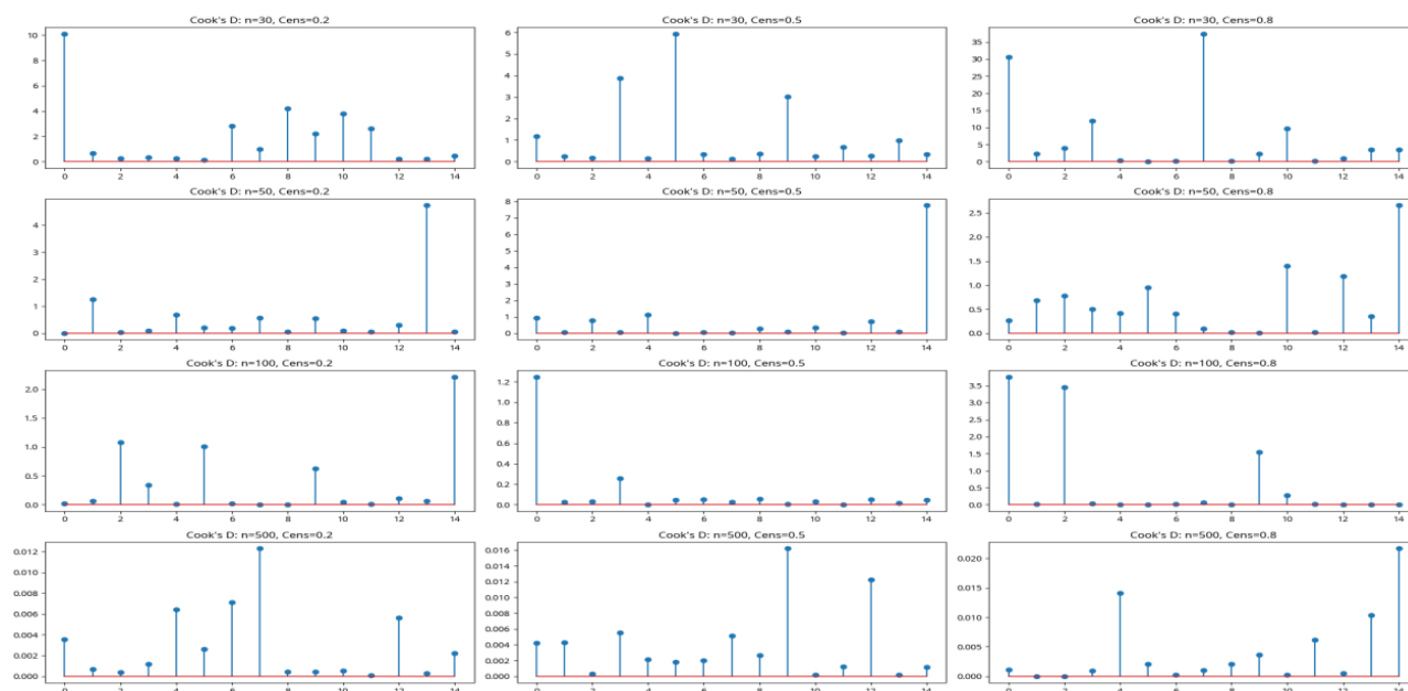
Akash Cook's Distance Grid - Case 1
