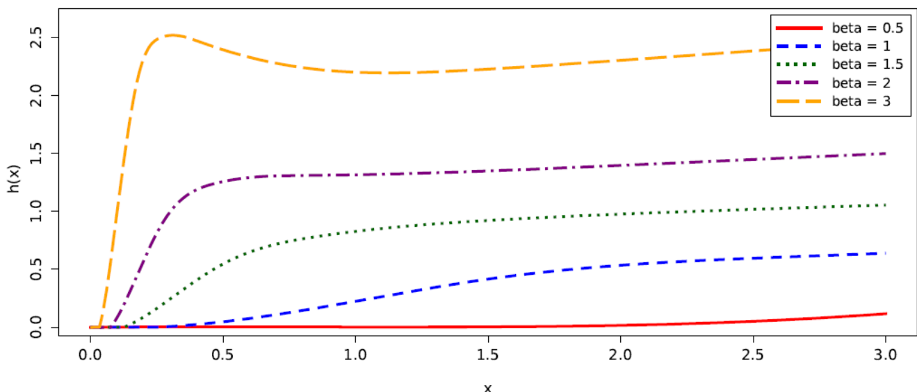
Figure 4. the hazard rate function at different value of parameter.
