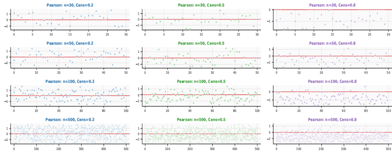
Figure 13. Pearson residuals for Case 3 across different sample sizes and censoring levels.
