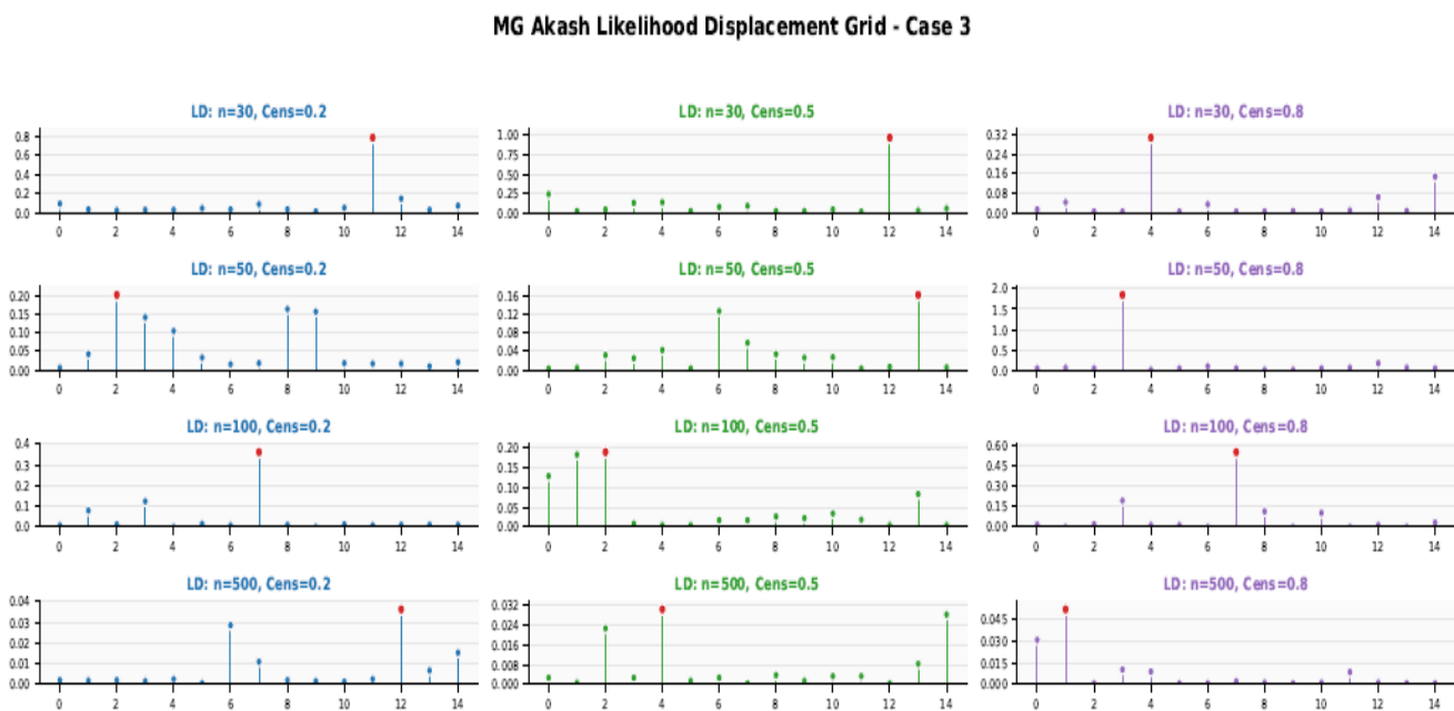
Figure 15. Likelihood displacement (LD) Case 3 across different sample sizes and censoring levels.
