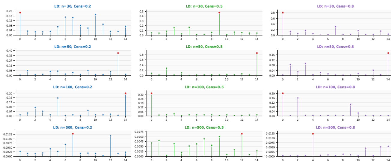
Figure 8. Likelihood Displacement (LD) for Case 1 under different sample sizes and censoring levels.
