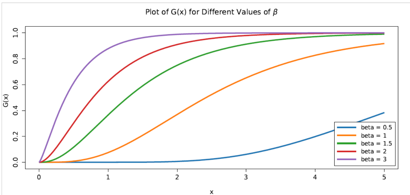
Figure 1. CDF of Minimum Guarantee Akash) Distribution at different value.
