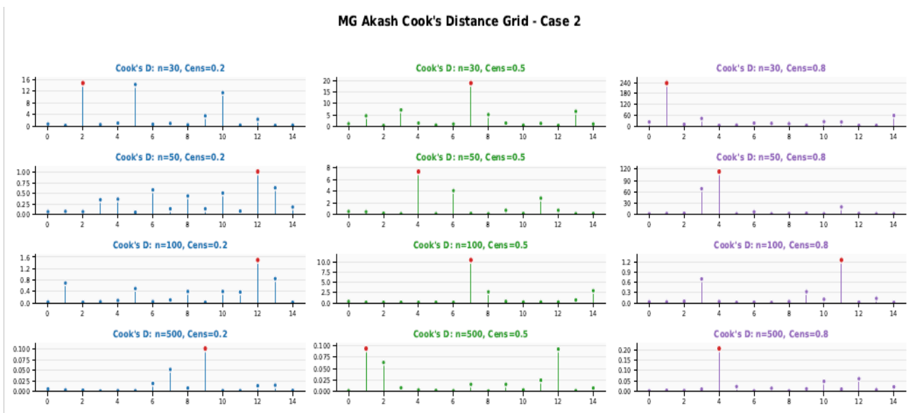
Figure 11. Cook's Distance values under Case 2 for different sample sizes and censoring levels.
