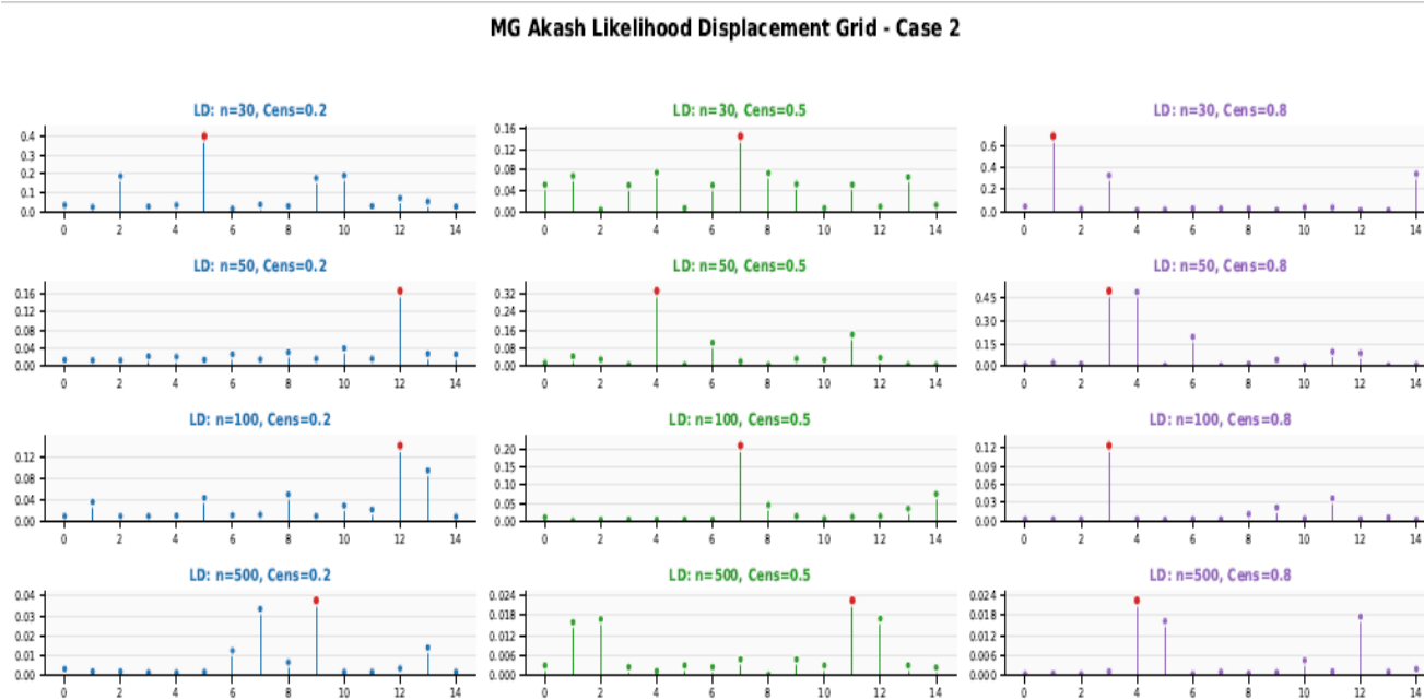
Figure 12. Likelihood Displacement (LD) values under Case 2 for different sample sizes and censoring levels.
