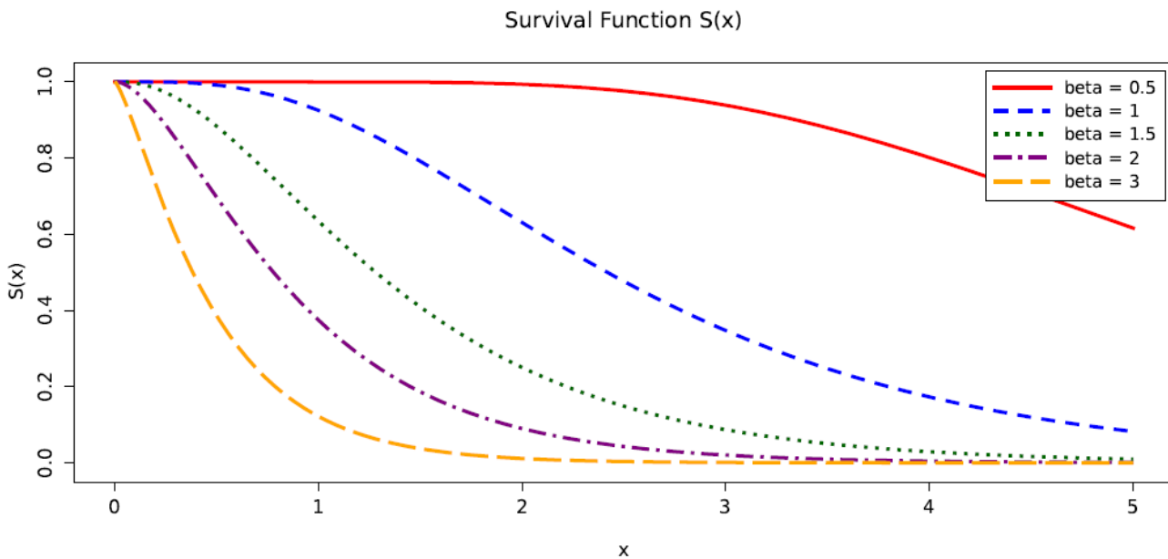
Figure 3. Survival Function of Minimum Guarantee Akash (MGA) Distribution at different value.
