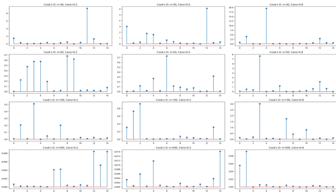
Figure 16. the Cook's Distance grid for Case 3 across different sample sizes and censoring levels.
