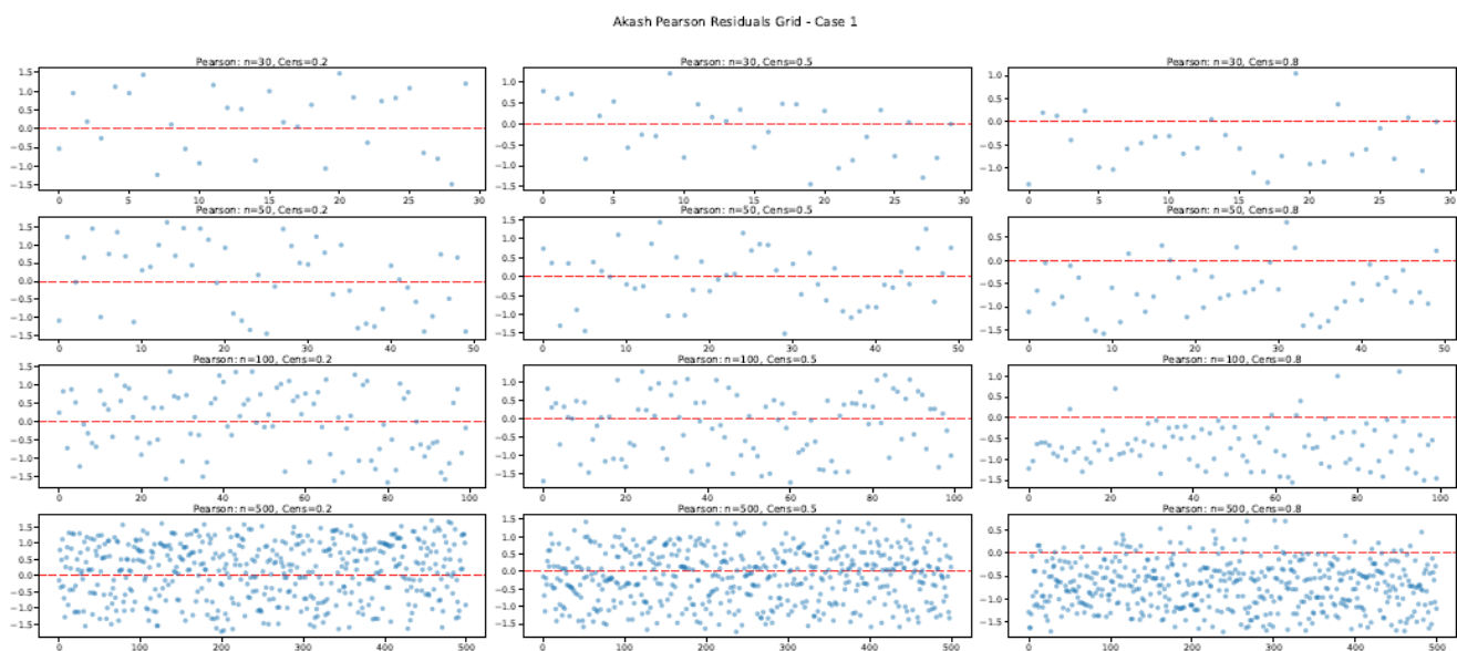
Figure 5. Pearson residuals for the MG Akash Regression Model (Case 1) across different sample sizes and censoring levels.
