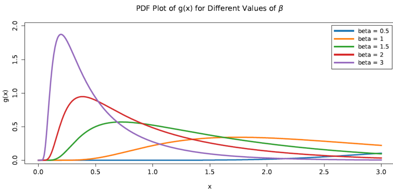
Figure 2. pdf of Minimum Guarantee Akash Distribution at different value.
