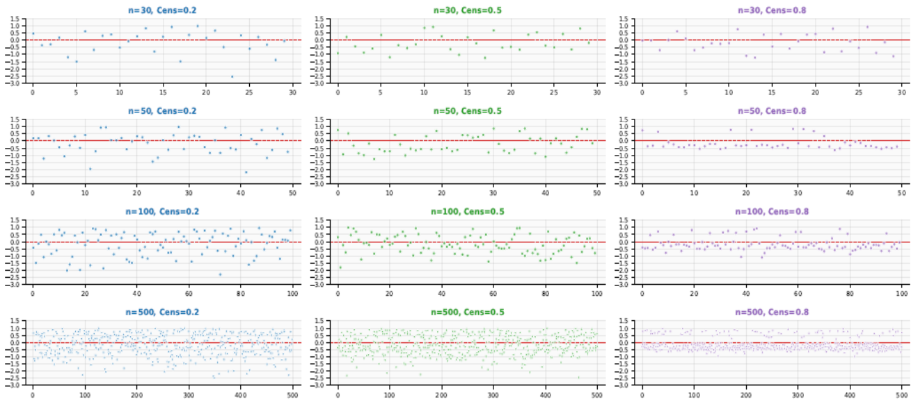
Figure 10. Martingale Residuals for Case 2 across different sample sizes and censoring levels.
