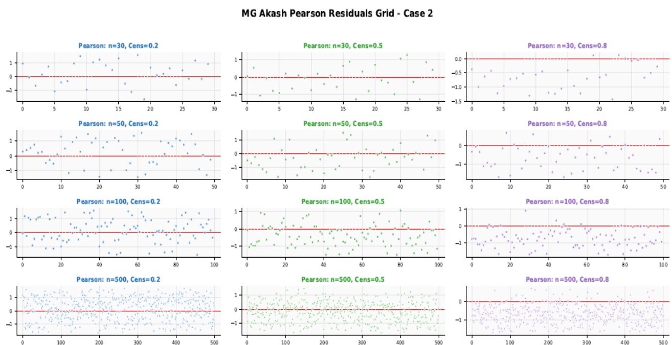
Figure 9. Pearson Residuals for Case 2 across different sample sizes and censoring levels.
